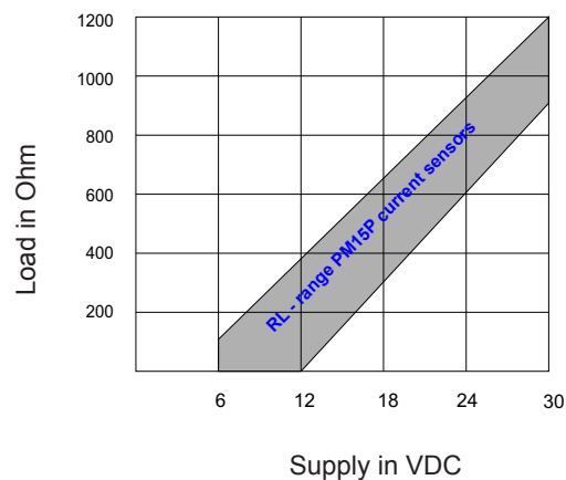
Load for 0(4)...20mA current version
